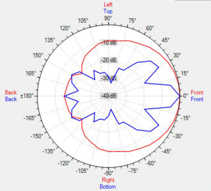
Data Shown: COLW41 (Apart Audio) Display Parameters: Frequency: 2000Hz (1/24th Octave)
