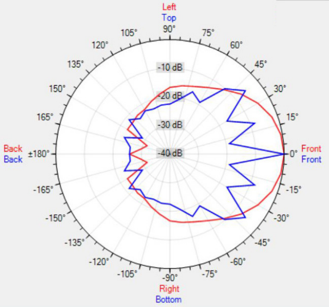
Data Shown: COLW41 (Apart Audio) Display Parameters: Frequency: 4000Hz (1/24th Octave)
