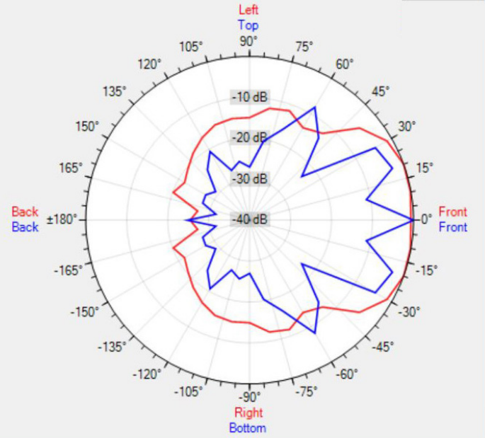
Data Shown: COLW41 (Apart Audio) Display Parameters: Frequency: 8000Hz (1/24th Octave)
