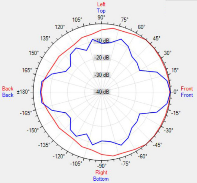
Data Shown: COLW41 (Apart Audio) Display Parameters: Frequency: 1000Hz (1/24th Octave)
