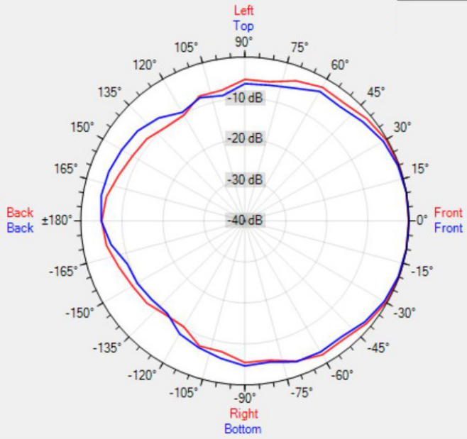
Data Shown: OVO5T (Apart Audio) Display Parameters: Frequency: 1000Hz (1/24th Octave)
