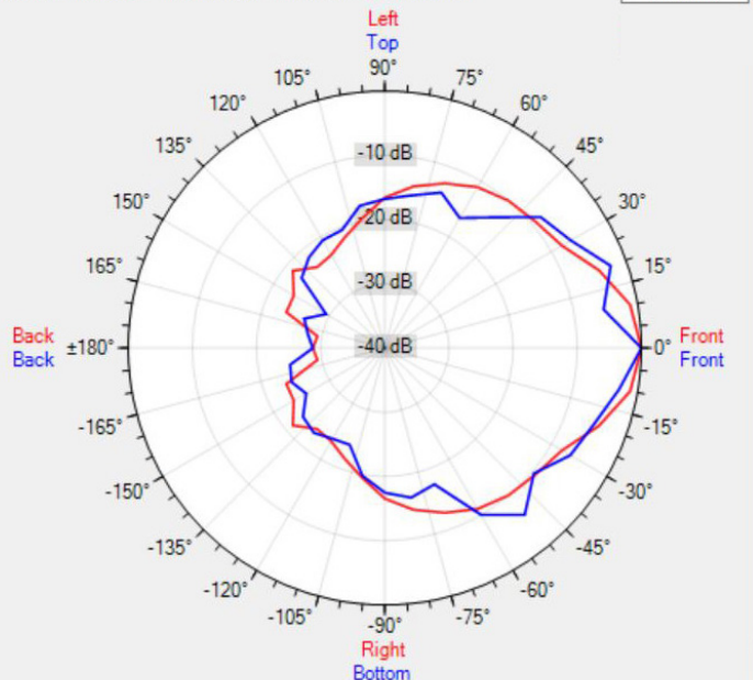
Data Shown: OVO5T (Apart Audio) Display Parameters: Frequency: 8000Hz (1/24th Octave)
