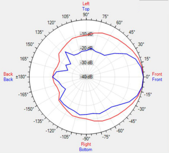
Data Shown: OVO5T (Apart Audio) Display Parameters: Frequency: 2000Hz (1/24th Octave)
