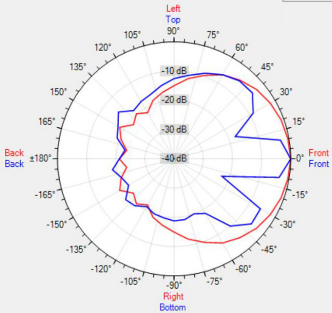
Data Shown: OVO5T (Apart Audio) Display Parameters: Frequency: 4000Hz (1/24th Octave)
